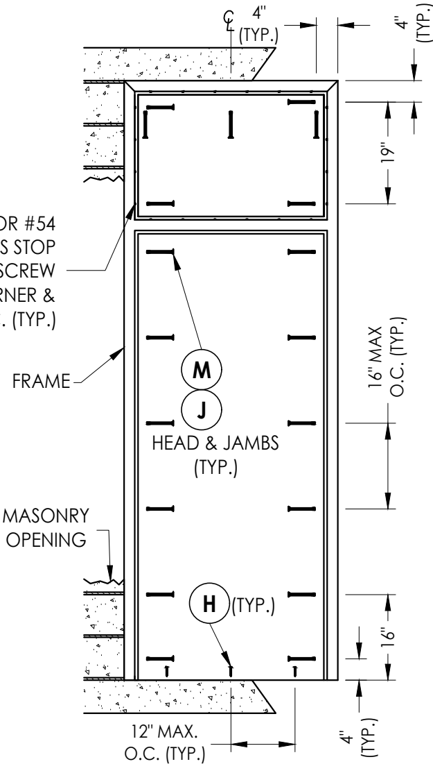
FRAME ANCHORING
